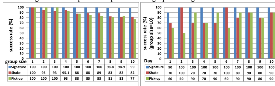
Fig. 3. User recognition success rate (in %) for various user target group sizes (left) and a detailed daily results for target group size of ten users (right).
